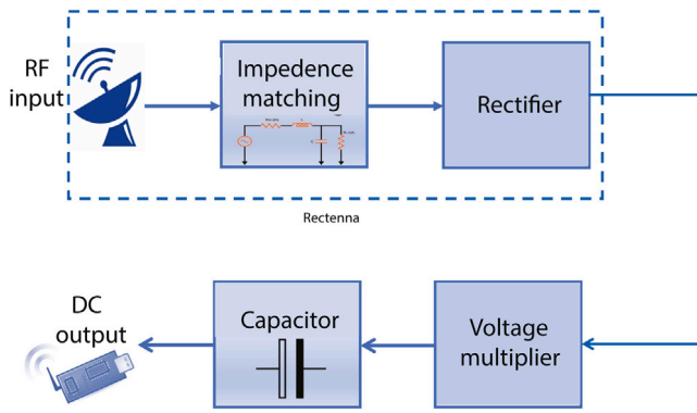
Fig. 7. Block diagram of a typical RF energy harvester.
